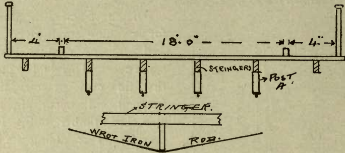
FIG. 56—SECTION OF A BRIDGE.
