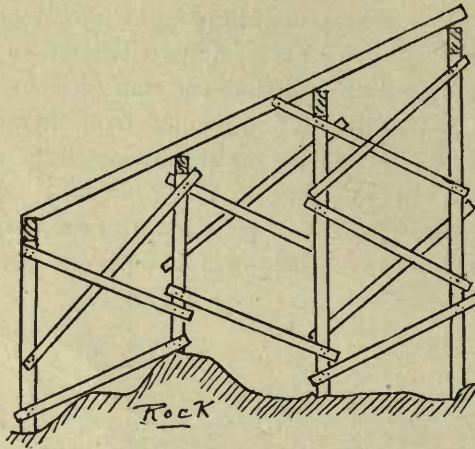
FIG. 41—SECTION OF A 25-FOOT STAND.
