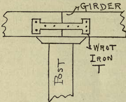
FIG. 35—A DOUBLE T STRAP ANCHOR.
