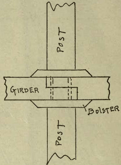
FIG. 36—A HALVED AND DOWELLED JOINT.
