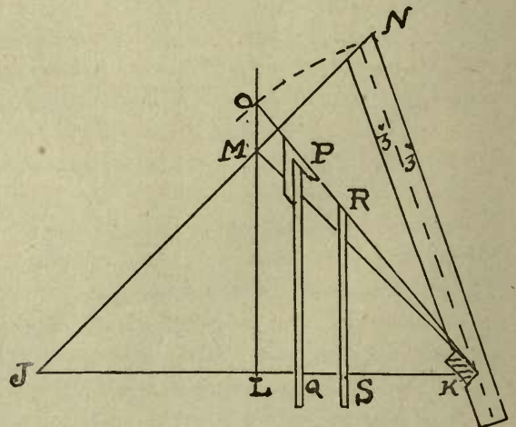
FIG. 1—PLAN AND LAYOUT OF A SIMPLE ROOF.
