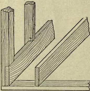
FIG. 3—FRAMING OF SILLS.
