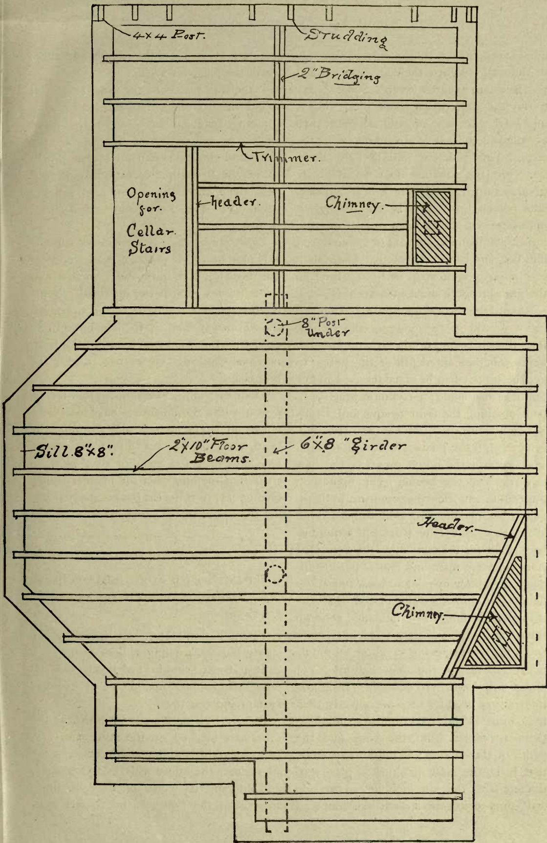
FIG. 11—FLOOR PLAN OF FIRST STORY TIMBERS.
