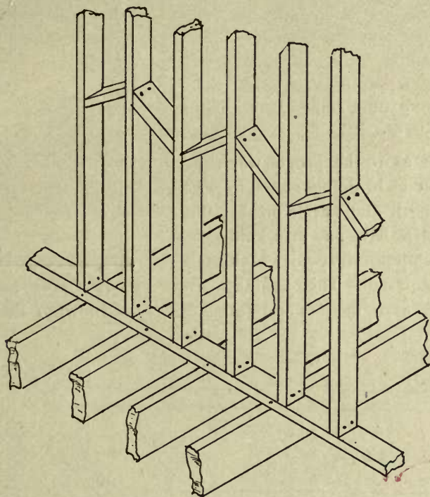
FIG. 13—A TRUSSED PARTITION.
