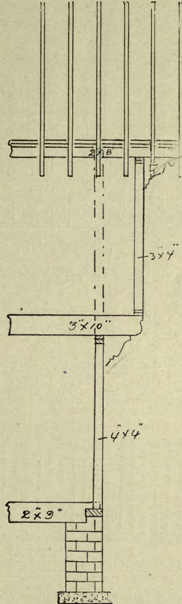
FIG. 49—SECTION OF STORIES.
