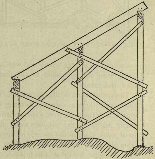
FIG. 40.—SECTION OF FRAMING OF A 20-FOOT STAND.
