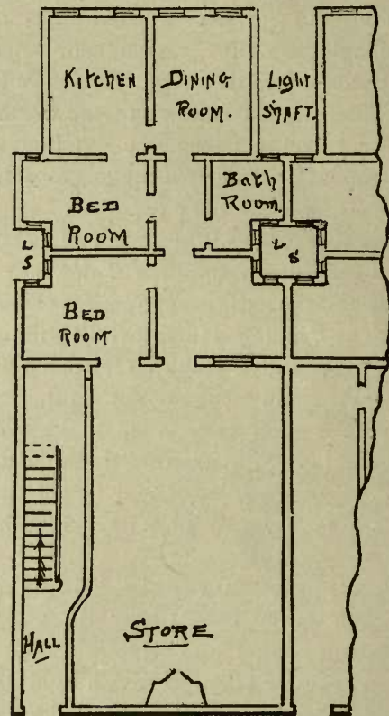
FIG. 30.—PLAN OF STORE FLOOR.
