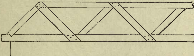
FIG. 61—LATTICE TRUSSINGS.
