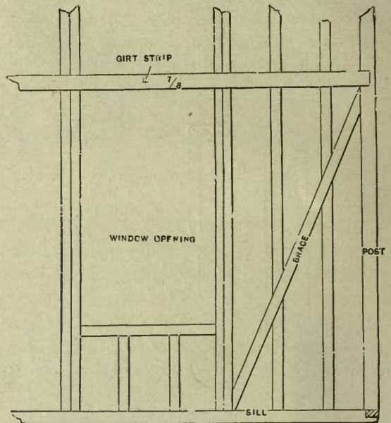
FIG. 7—ELEVATION OF A STUD WALL WITH BRACE.
