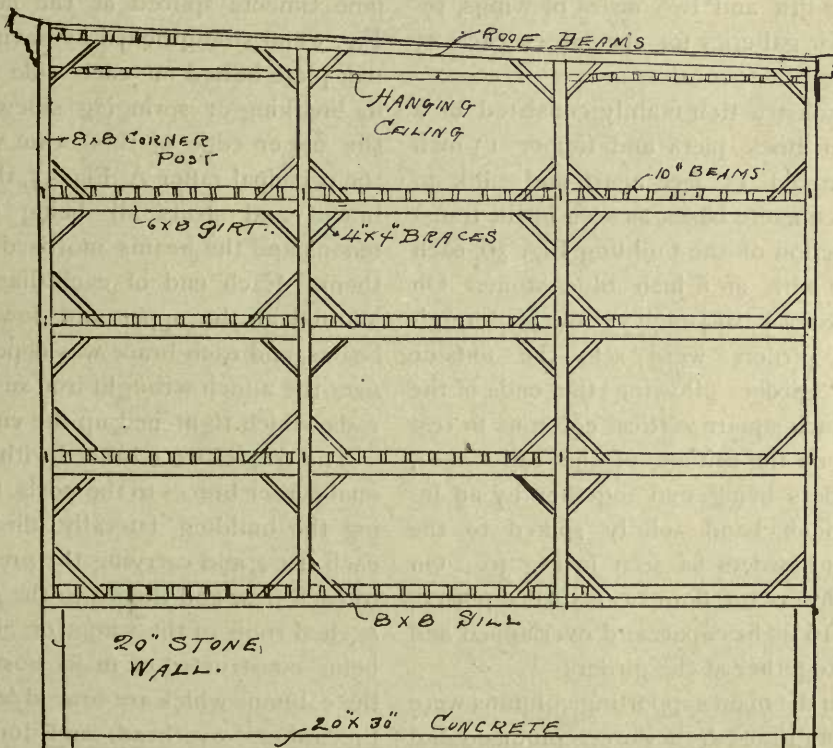
FIG. 34.—FRAMING OF GABLES AND PARTY WALLS.
