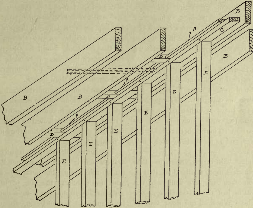
FIG. 20—FRAMING OF A PARTITION BETWEEN BEAMS.
