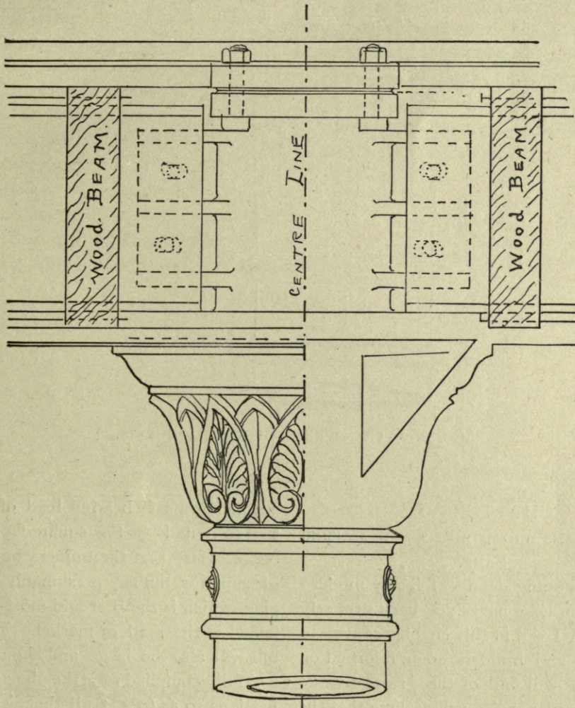
FIG. 28—LONGITUDINAL SECTION OF FLOOR.
