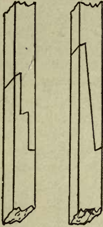
FIG. 31.—SPLICING POSTS.
