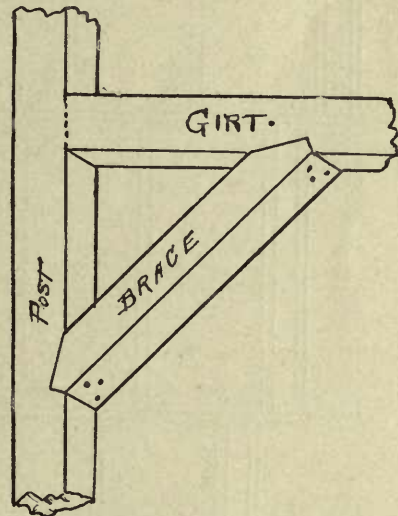
FIG. 32.—FRAMING OF BRACE.
