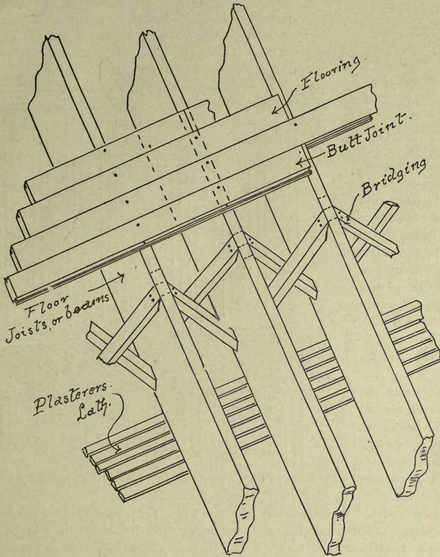
FIG. 18—PROJECTION OF A BALLOON FRAME FLOOR.
