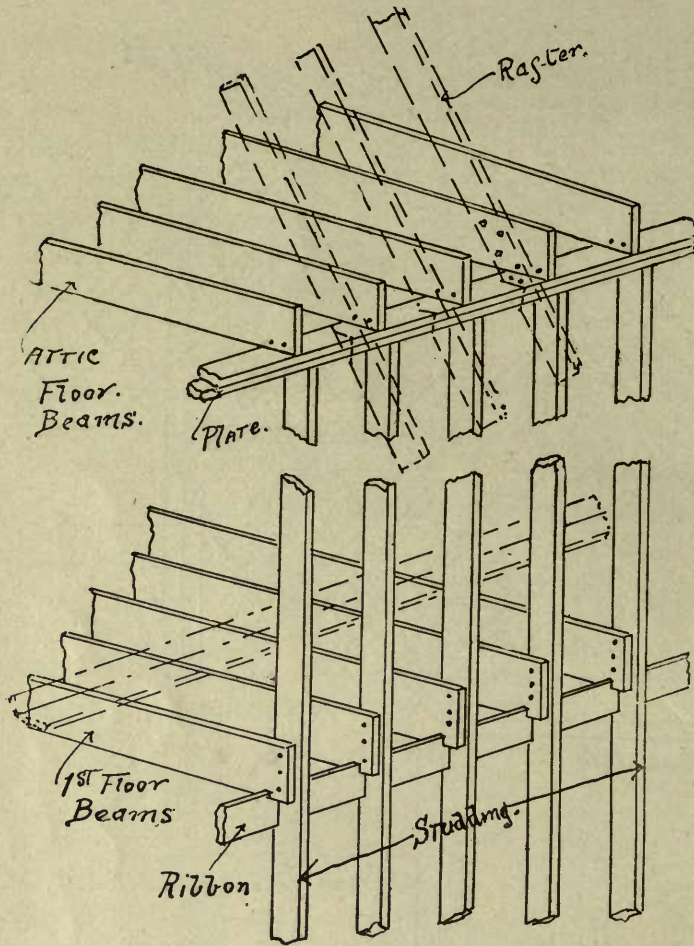
FIG. 9—FLOOR JOISTS, STUDS AND RAFTERS.
