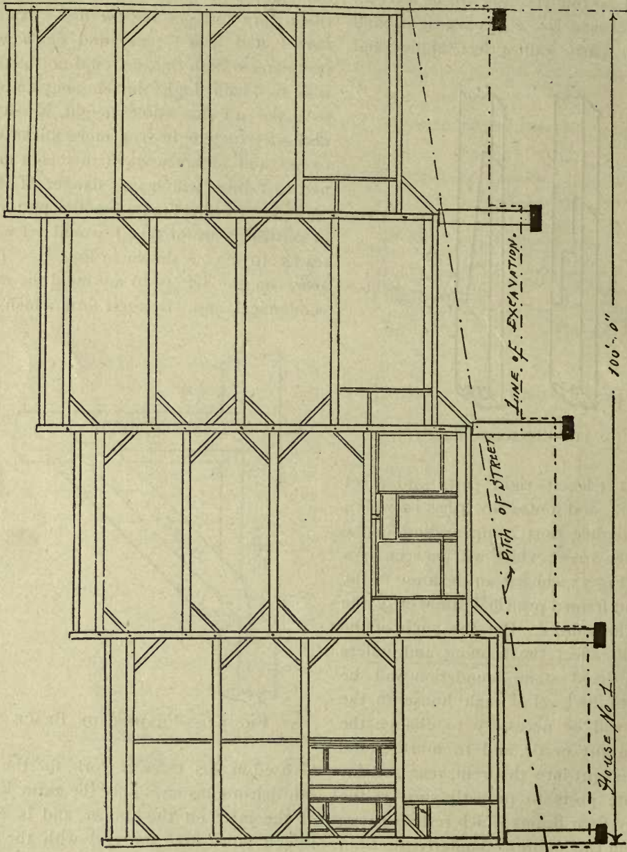
FIG. 33.—ELEVATION OF ANGULAR FRAMING.
