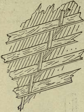
FIG. 14--BRIDGING OF FLOORS AND ROOFS.
