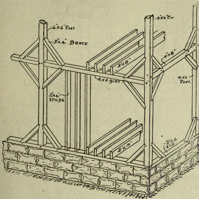
FIG. 22—PERSPECTIVE VIEW OF A BRACED FRAME.
