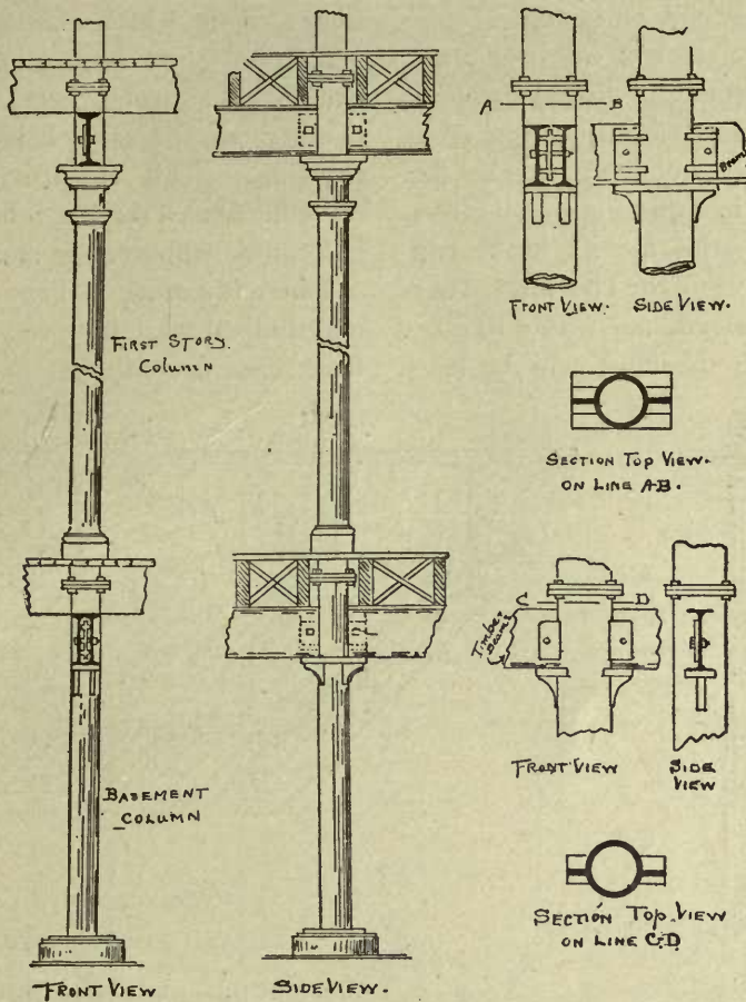
FIG. 23—ELEVATIONS AND DETAILS, WOOD AND IRON CONSTRUCTION.
