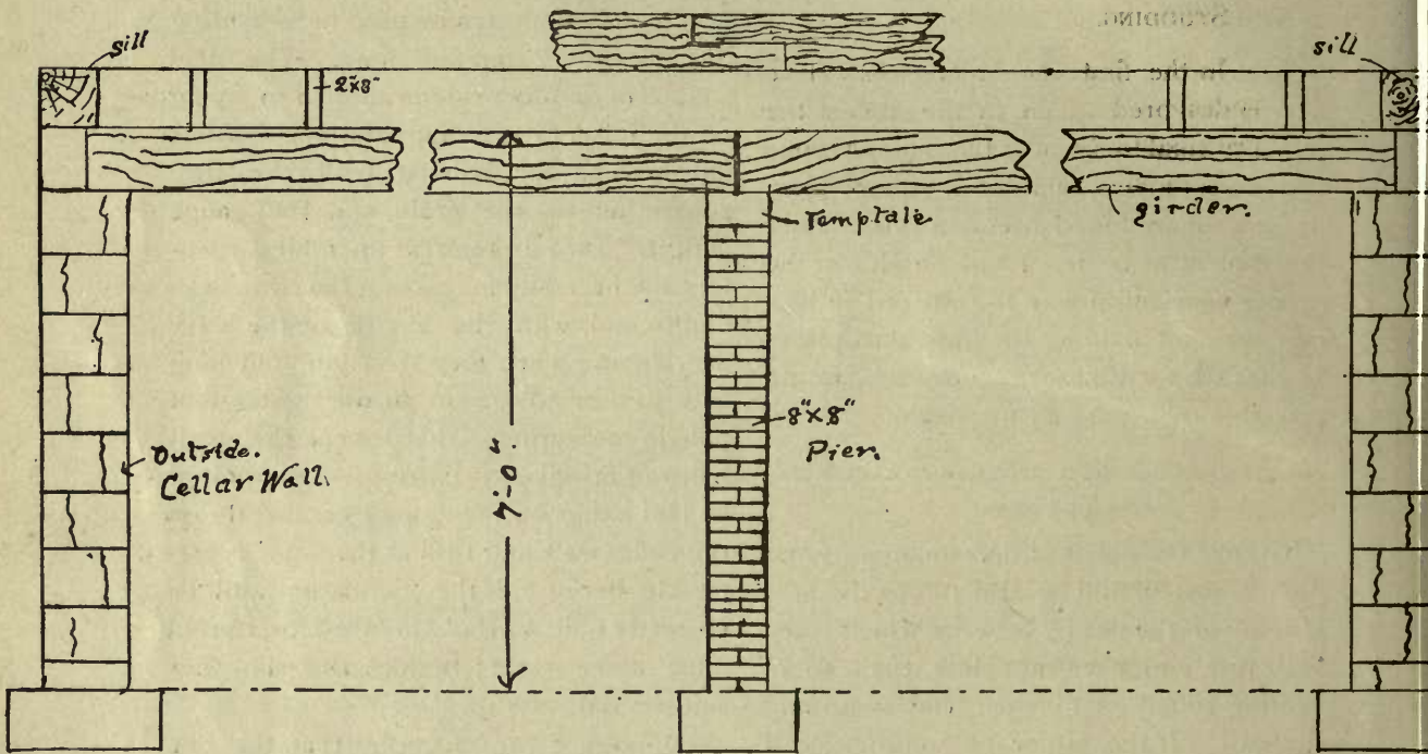
FIG. 10—VIEW OF CELLAR WALL, PIER GIRDER AND SILLS.
