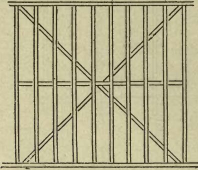
FIG. 50.—PARTITION BRACED DIAGONALLY.
