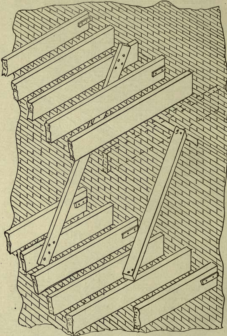
FIG. 12—METHOD OF BRACING BRICK WALLS.
