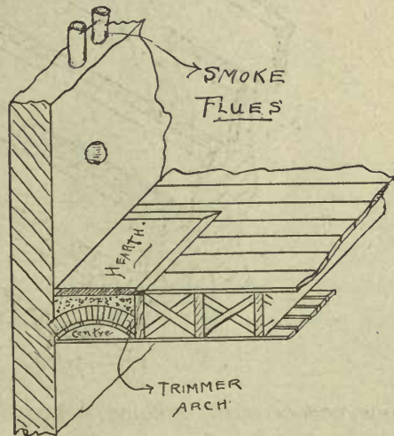
FIG. 11—SECTION THROUGH FLOOR AT HEARTH.
