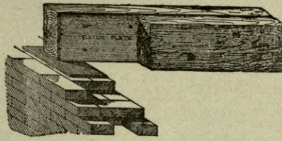
FIG. 27—FLITCH PLATE GIRDERS.
