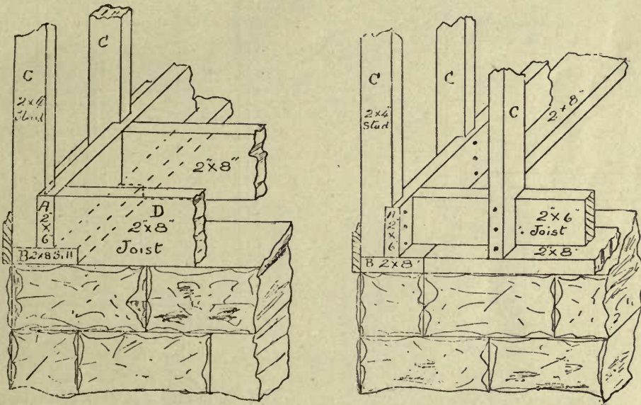
FIG. 5—TWO MORE EXAMPLES OF SILL CONSTRUCTION.
