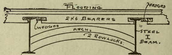
FIG. 26—SECTION SHOWING METHOD OF WEDGING BEARERS.
