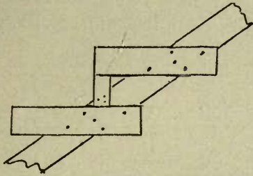
FIG. 44.—BRACKETS NAILED ON.
