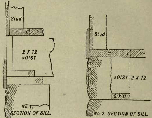
FIG. 4—CHEAP SILLS.
