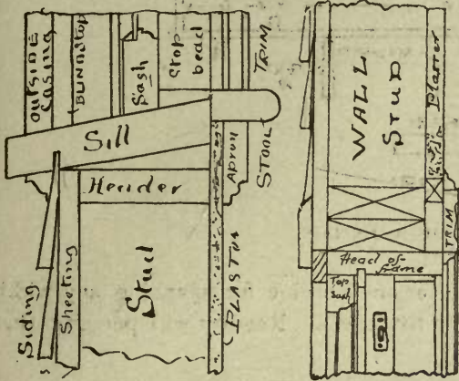
FIG. 53— SECTION OF SILL, ETC.
