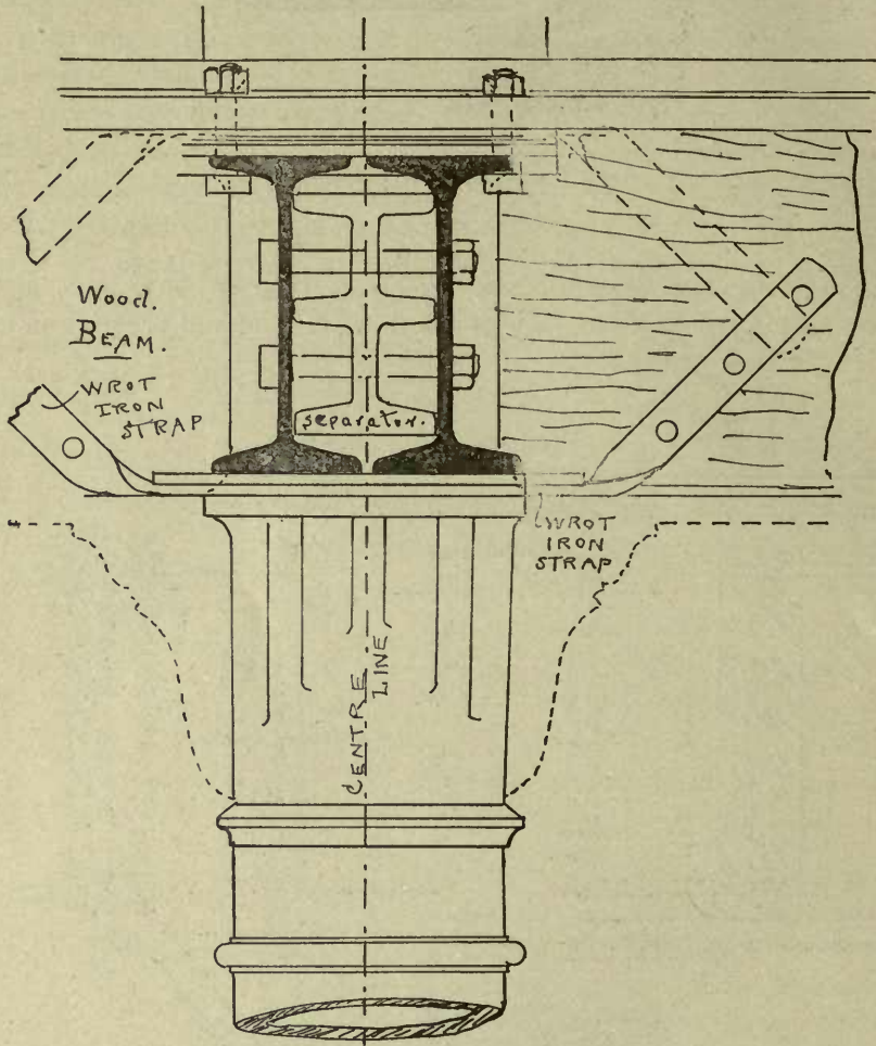
FIG. 29—TRANSVERSE SECTION OF FLOOR.
