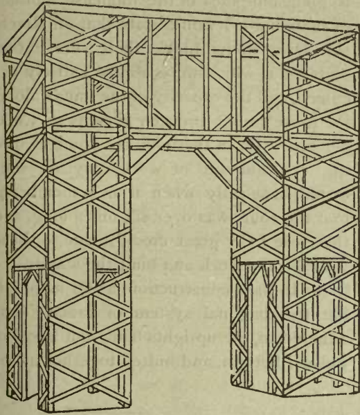
FIG. 39.—GENERAL VIEW OF FRAMING OF DEWEY ARCH.
