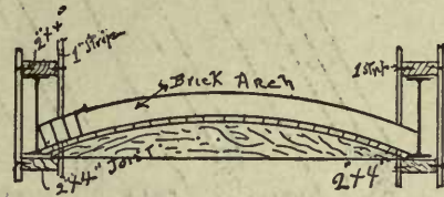
FIG. 5—METHOD OF SETTING CENTRES FOR FIREPROOF FLOORS.
