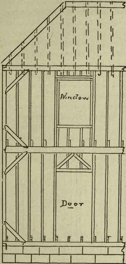
FIG. 25—SIDE VIEW OF BRACED FRAME.
