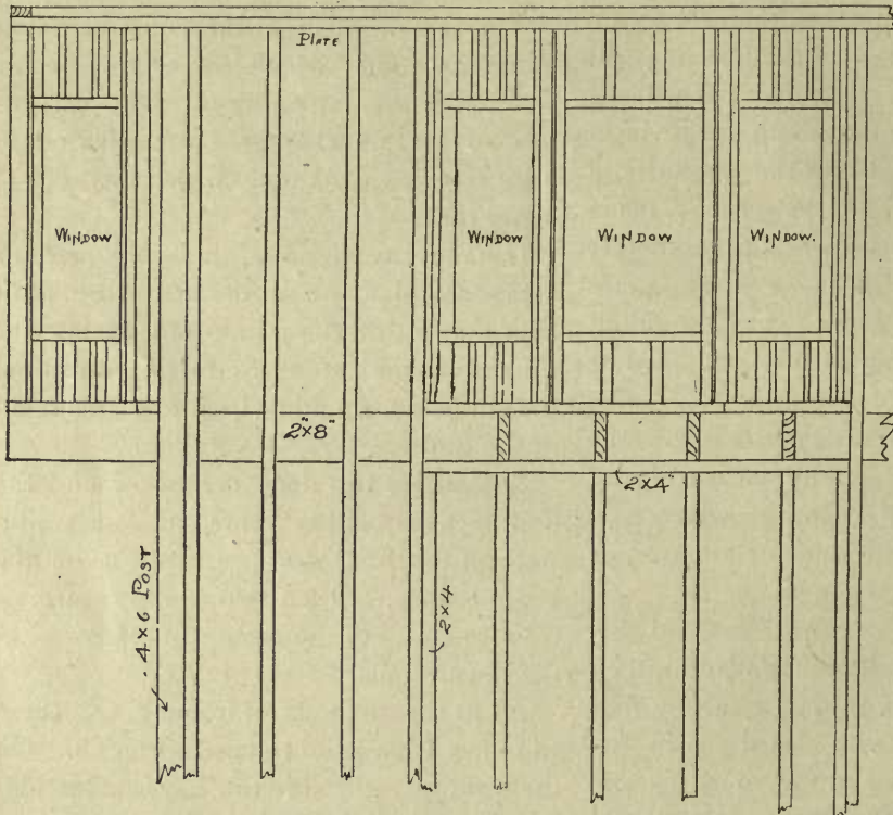
FIG. 29—ELEVATION.
