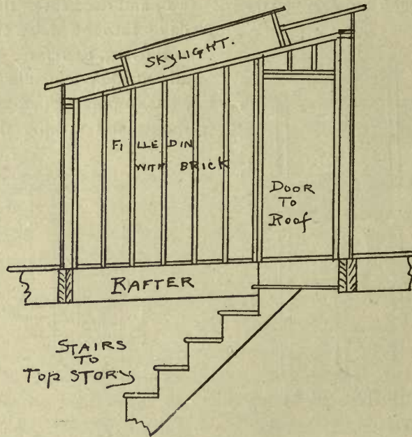
FIG. 21—SECTION OF BULKHEAD.
