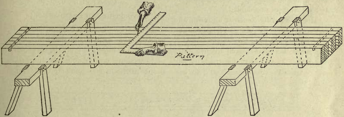
FIG. 14—LAYING OUT BEAMS WITH THE STEEL SQUARE.
