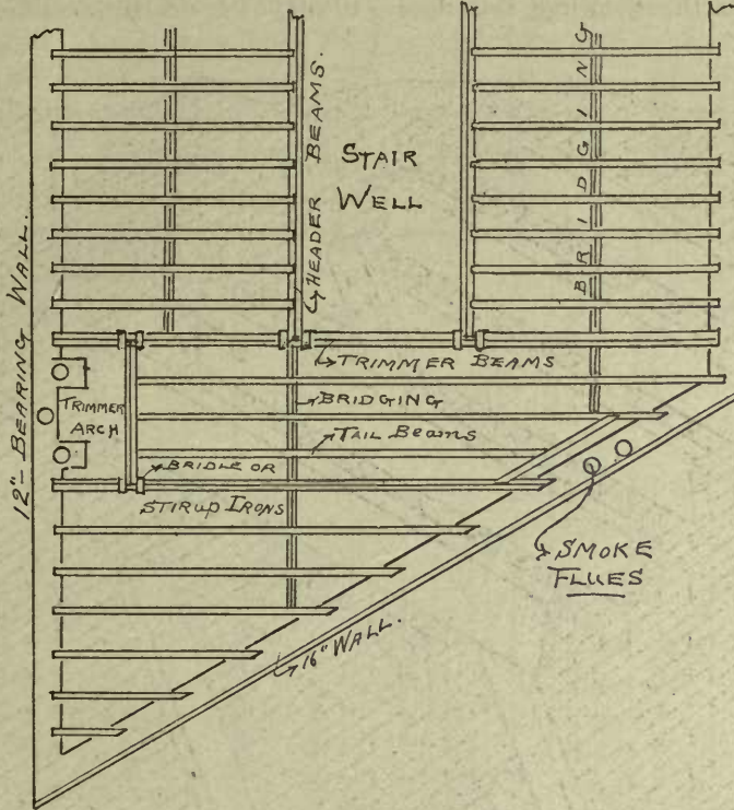
FIG. 10—FRAMING PLAN OF A BRICK CITY HOUSE.
