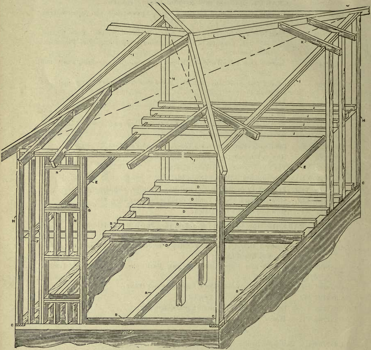
FIG. 1—SKELETON VIEW OF A BALLOON FRAME.
