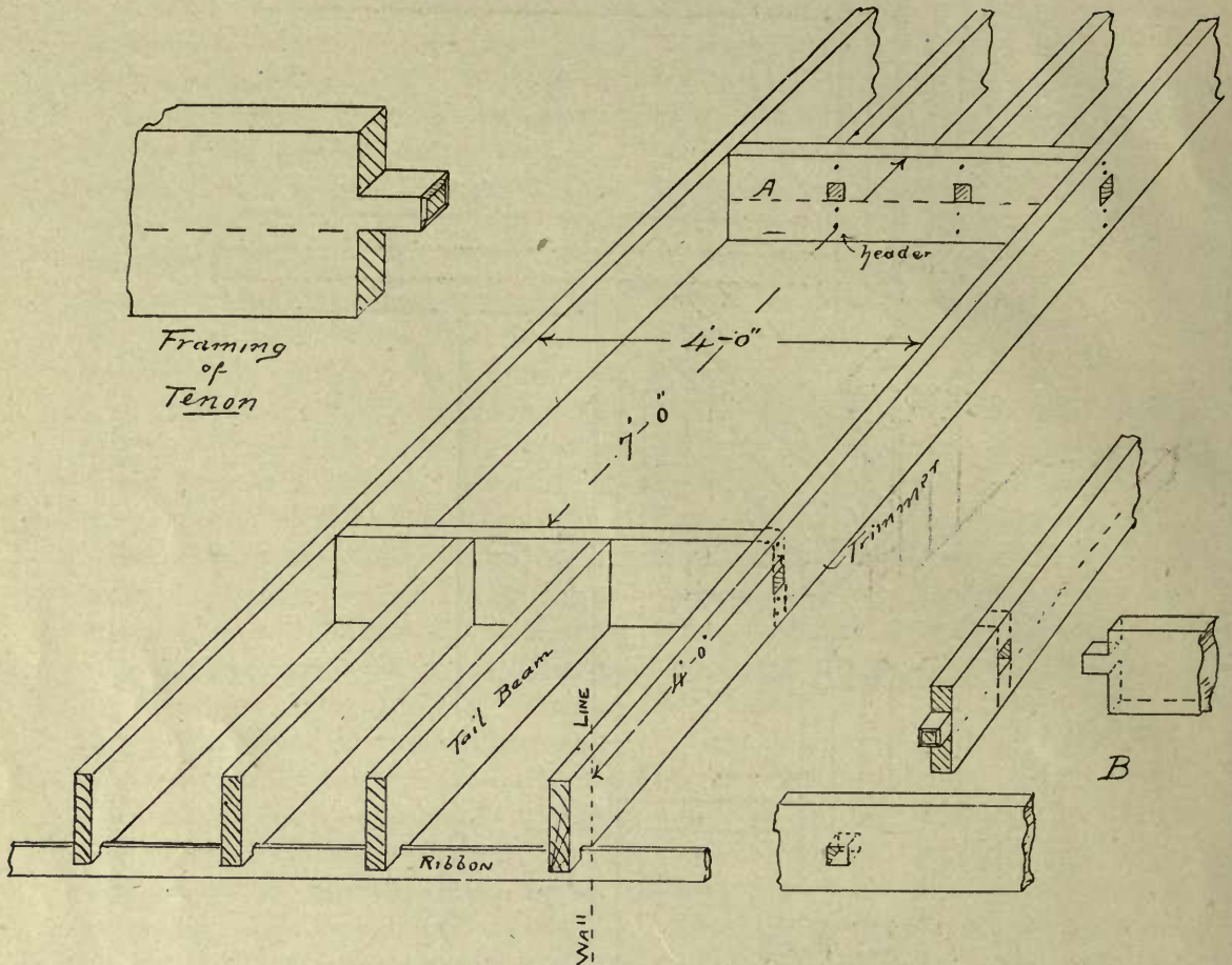
FIG. 13—FRAMING OF A WELL HOLE.
