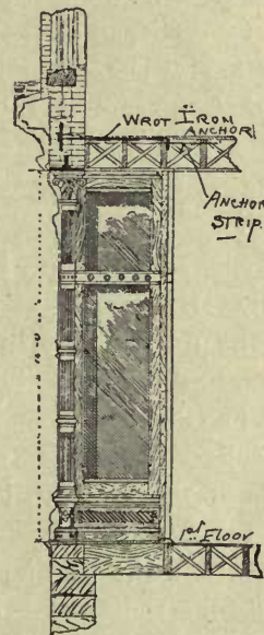
FIG. 8—SECTION OF FRONT OF STORE, SHOWING ANCHORS, STRIPS, BEAMS, ETC.
