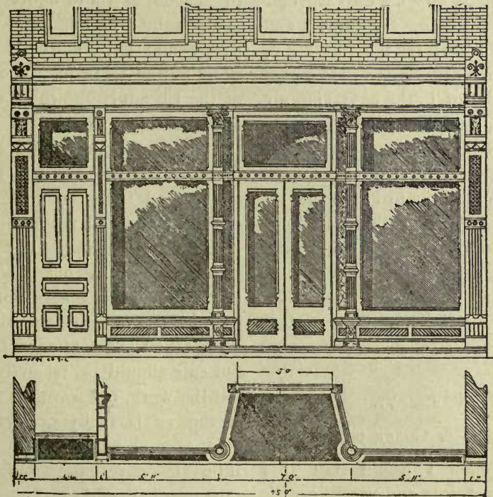
FIG. 22-A—ELEVATION AND PLAN OF STORE FRONT.
