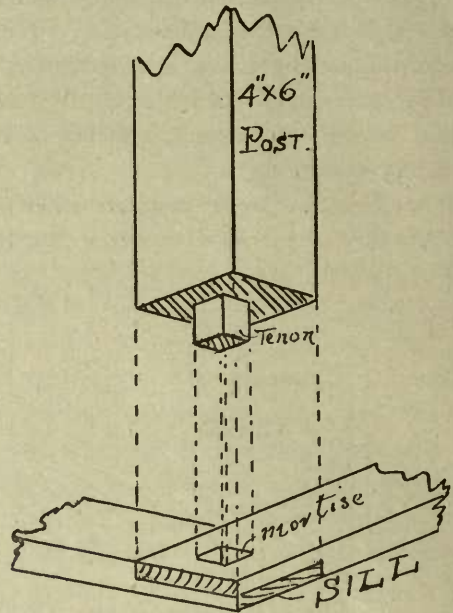
FIG. 23—FRAMING OF POST AND SILL.
