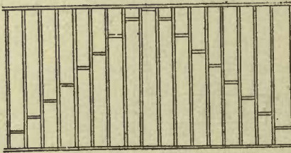
FIG. 51.—BRACING A LONG PARTITION.
