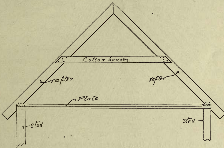
FIG. 16—ELEVATION OF A COLLAR BEAM ROOF.
