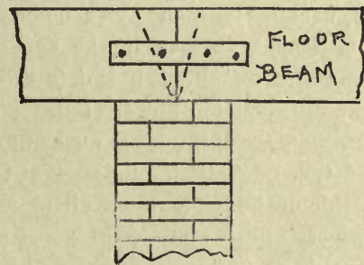
FIG. 34—A STRAP ANCHOR NAILED ON.
