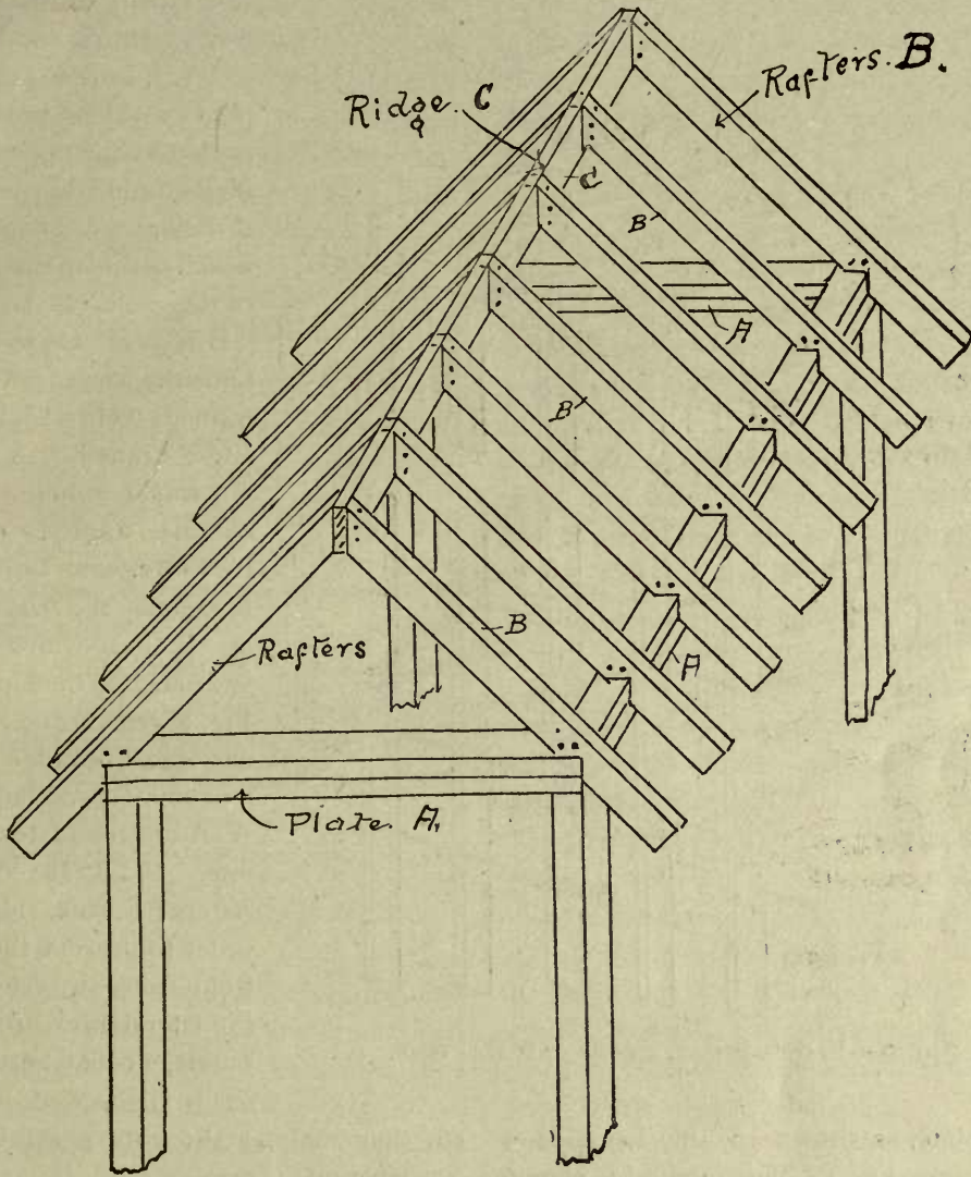
FIG. 8—ROOF TIMBERS SET UP.
