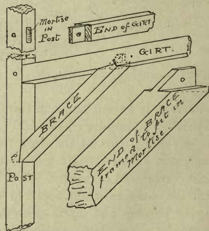
FIG. 24—FRAMING OF GIRT AND BRACE.
