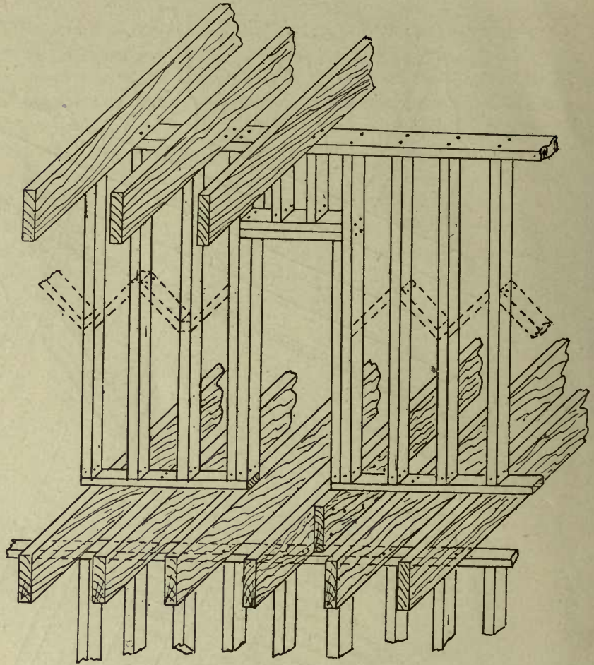
FIG. 19—A FRAMED INSIDE PARTITION.
