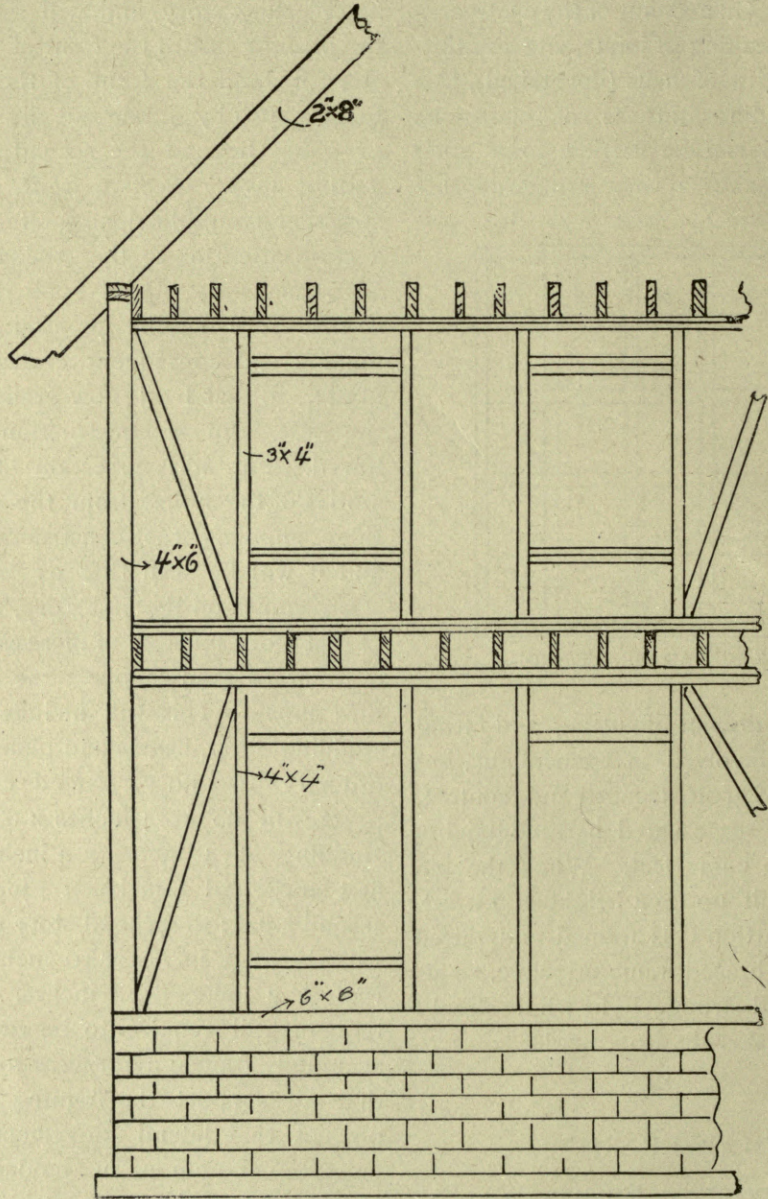
FIG. 48—FRONT VIEW OF FRAMING.
