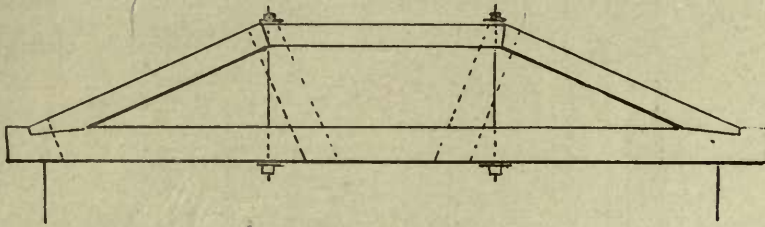
FIG. 59—SIMPLE TRUSSED BRIDGES.
