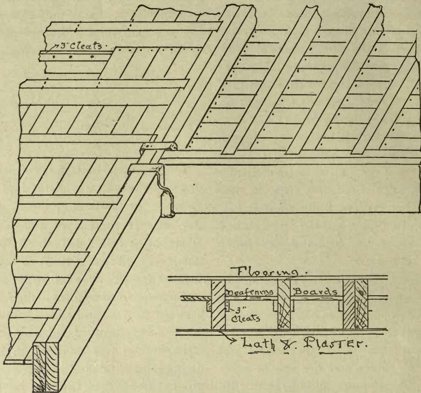
FIG. 18—METHOD OF DEAFENING FLOOR.
