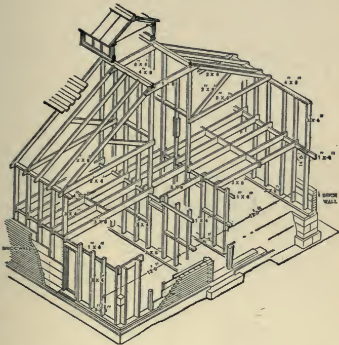
BALLOON FRAME FOR SIDING ROUGH CAST ON BRICK-CLAD.
